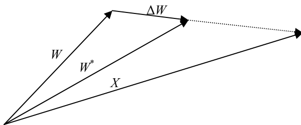
Figure 2. Weight correction of winning neurons
