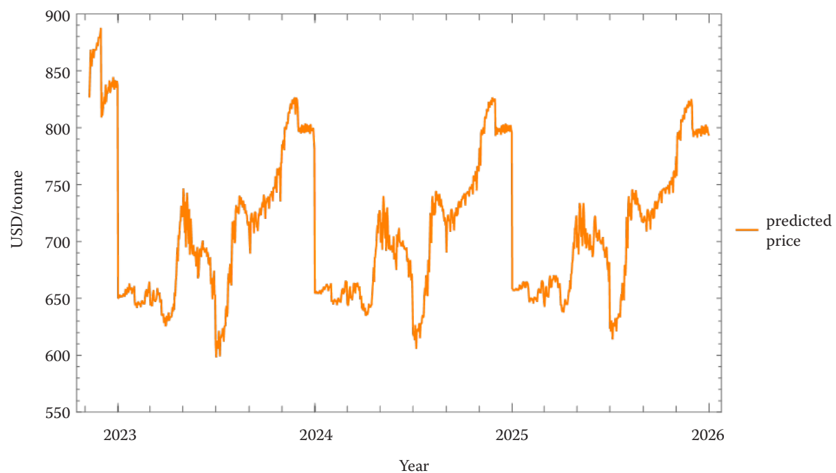
Figure 7. Price prediction
